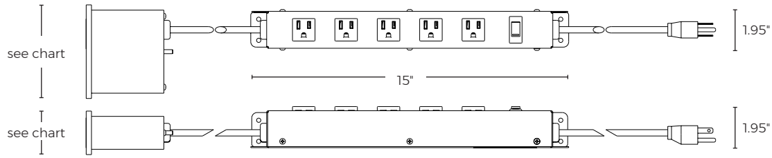
5-outlet power strip model shown
